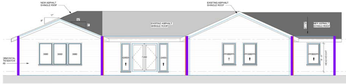
Front Elevation
